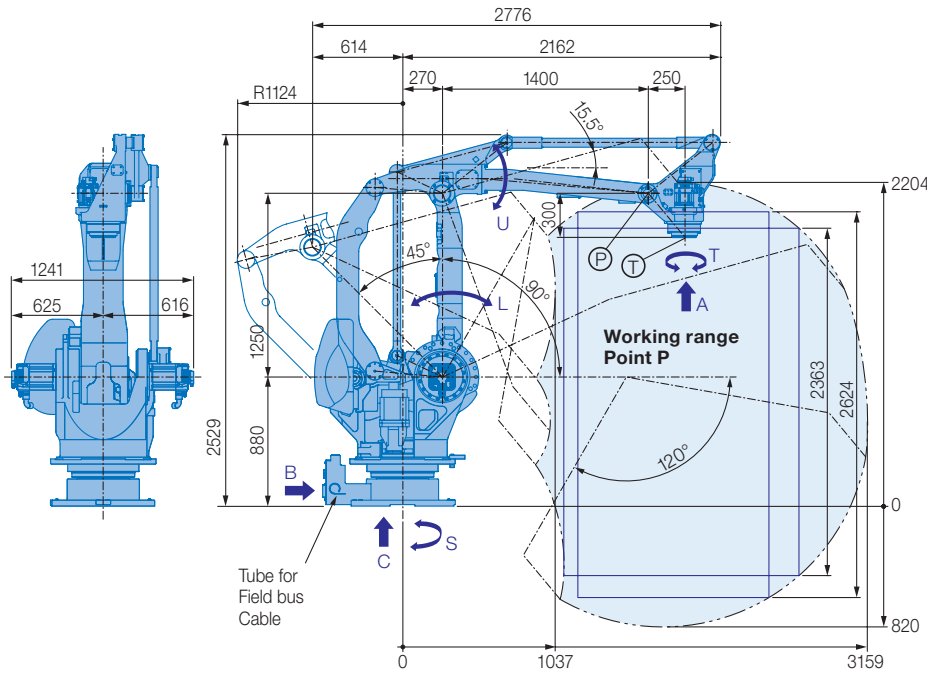
View A
